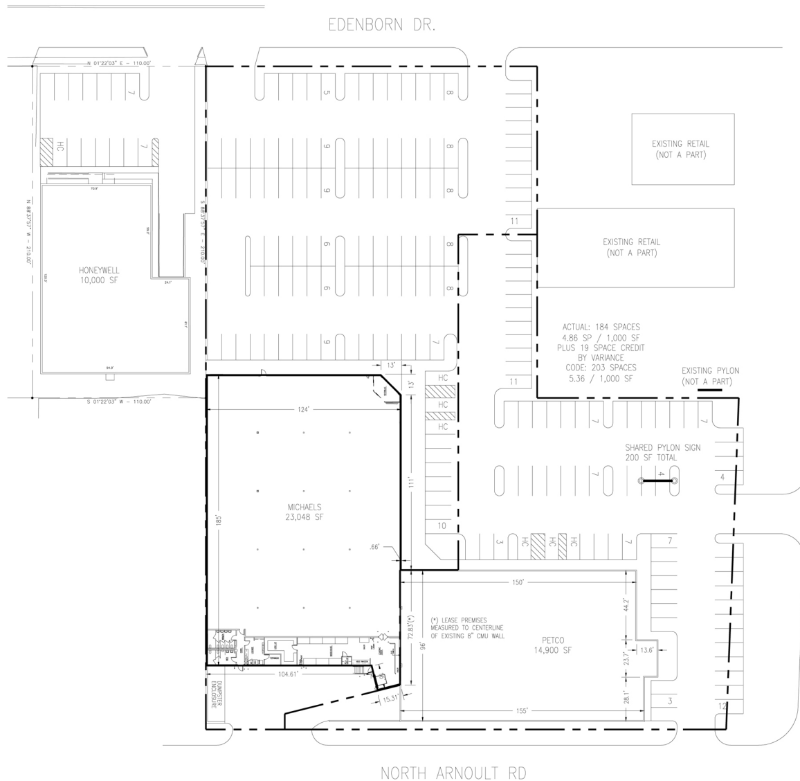
1 DEVELOPMENT SITE PLAN 1" = 30'-0" (22 x 34) OR 1" = 60" (11 x 17)
